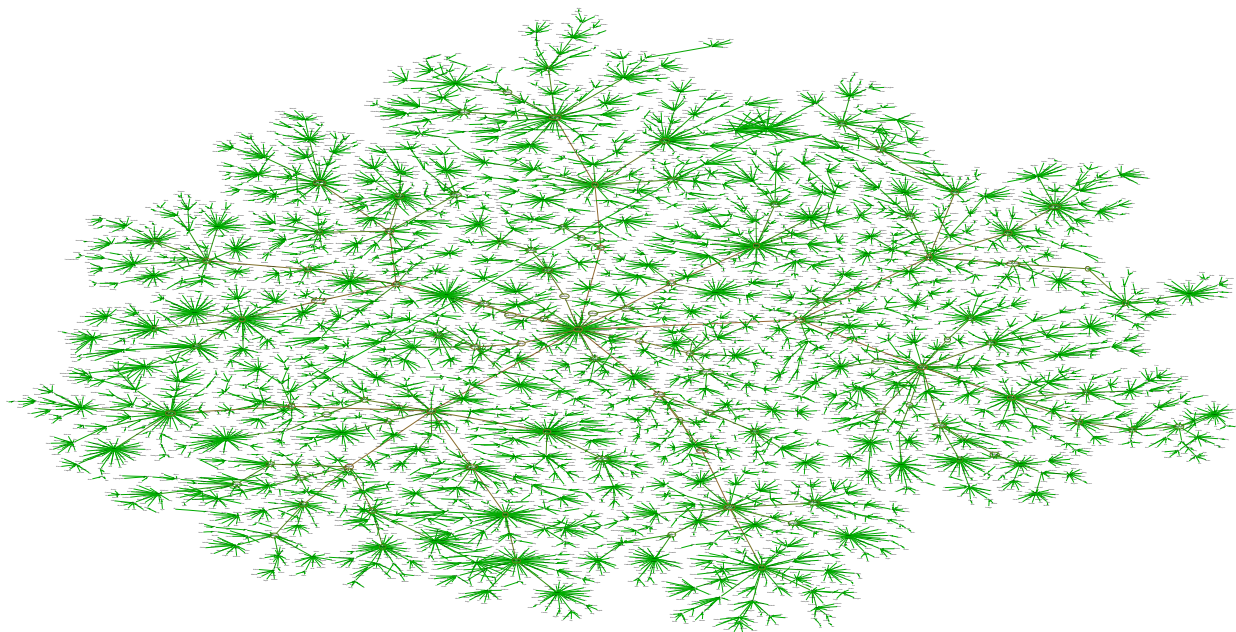
The third largest tree in the Mathematical Genealogy Project. Total 10018 mathematicians. Arrows point from a mathematician to his/her supervisor. Top 100 mathematicians with the most "off-springs" are circled. Data acquired in 2008. Produced by Yifan Hu, AT&T Labs Research.
