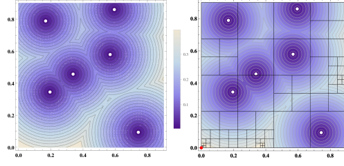
Fig. 4. Left: contour plot of the distance to a set of six (white) points in the space [0, 0.9] \times [0, 0.9] . There are seven or more local maxima. E.g., near \{0, 0.55\} and \{0.4, 0.7\} . Right: an illustration of the quadtree structure generated during our algorithm for finding the global optimal embedding of a node that is farthest away from the set of six points. The final solution is \{0, 0\} (red point).
